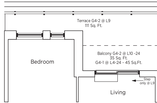
TERRACE PLAN SUITE G4-2 AT LEVEL 9
