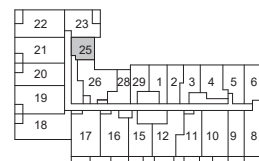
FLOOR 7 UNIT 725 SLAB TO SLAB HEIGHT 9'0"
